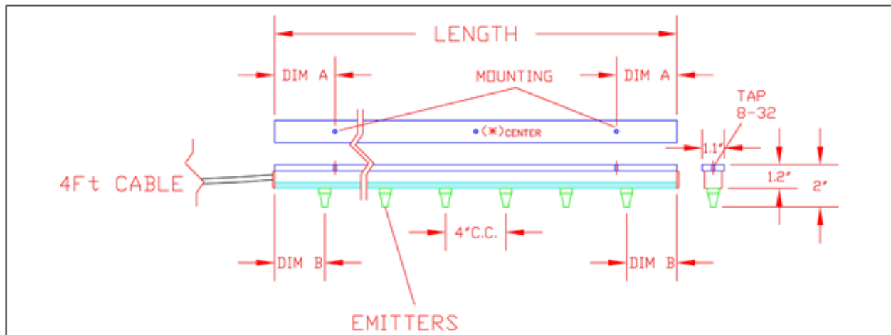
Figure 3. EMIT Non-Air Assisted Ion Bar dimensions
